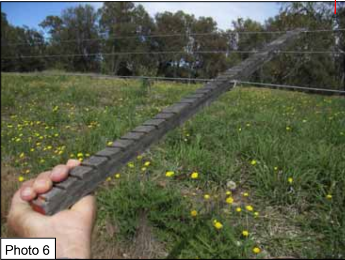
Photos 3-6: Wires are not run through the star pickets themselves but are attached to the pickets on the downstream side of expected flood flows (photos 3 & 4 above). The wire will be more likely to release from the picket if it is struck by debris, rather than pulling the star picket out. Photo 5 (bottom left) shows a close-up of a galvanized earth spike. Proper earthing of electric fencing is vital to ensure maximum performance and a minimum of three, inter-connected 2m long earth spikes should be fitted. Photo 6 (bottom right) shows how flexible the fence is where droppers are used - this allows debris to flow through the fence with less likelihood of it snagging the wires. This type of fence is ideal for situations where flood flow direction is unpredictable.
